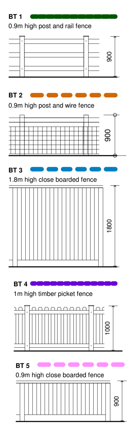
Boundary Treatments 1 : 50
